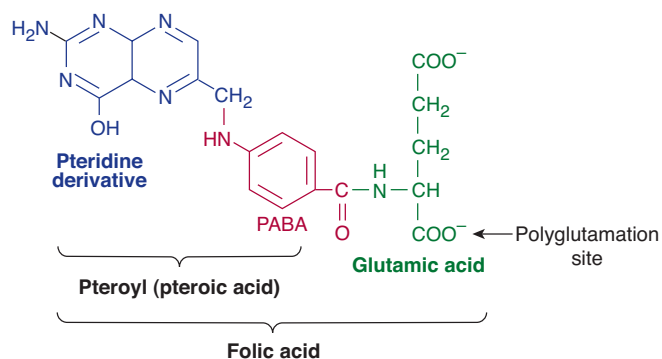
FIGURE 33–4 The structure of folic acid. (Reproduced, with permission, from Murray RK et al: Harper's Biochemistry , 24th ed. McGraw-Hill, 1996.)
