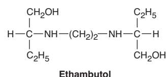
Ethambutol
