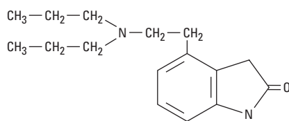
Ropinirole
