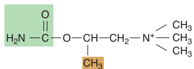
Bethanechol (carbamoyl- \beta -methylcholine)
