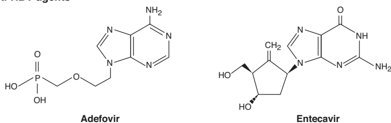
FIGURE 49-2 Chemical structures of some antiviral nucleoside and nucleotide analogs.
