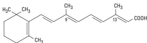
Retinoic acid
