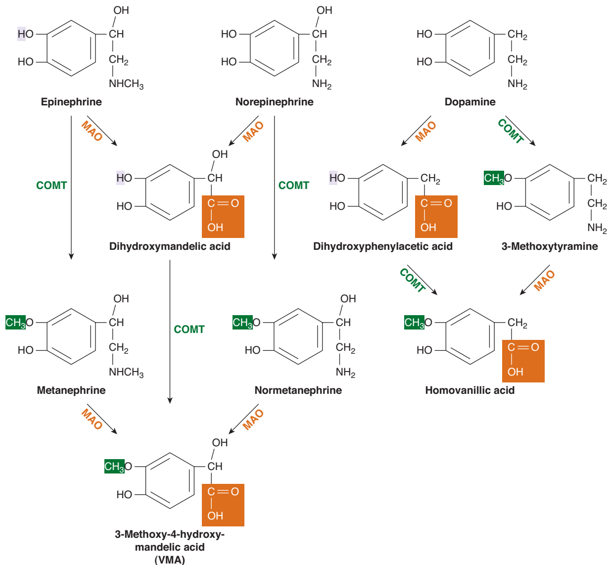
FIGURE 6-6 Metabolism of catecholamines by catechol-O-methyltransferase (COMT) and monoamine oxidase (MAO). (Modified and reproduced, with permission, from Greenspan FS, Gardner DG [editors]: Basic and Clinical Endocrinology , 7th ed. McGraw-Hill, 2003.)
