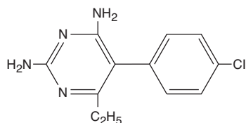
Pyrimethamine
