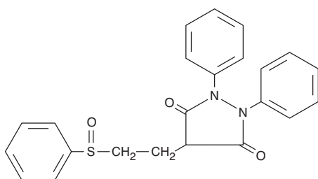
Sulfapyrazone
