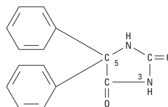
Phenytoin
