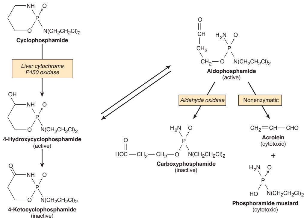
FIGURE 54-5 Cyclophosphamide metabolism.
