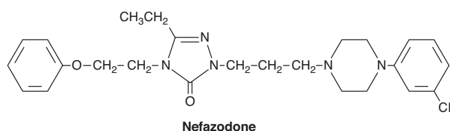
FIGURE 30-4 Structures of the tricyclic antidepressants (TCAs).
