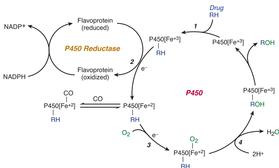
FIGURE 4–3 Cytochrome P450 cycle in drug oxidations. RH, parent drug; ROH, oxidized metabolite; \text{e}^- , electron.
