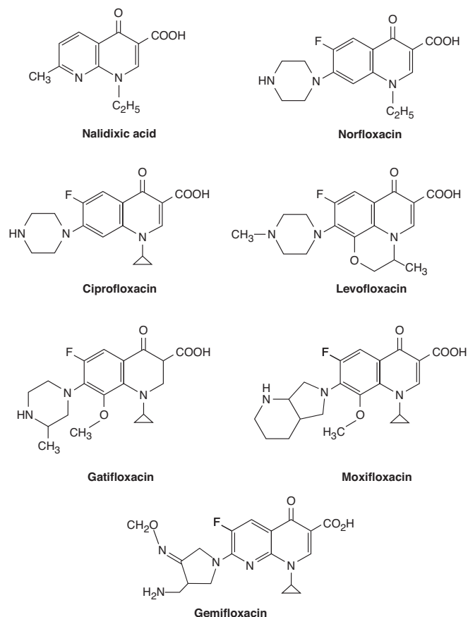
FIGURE 46-3 Structures of nalidixic acid and some fluoroquinolones.
